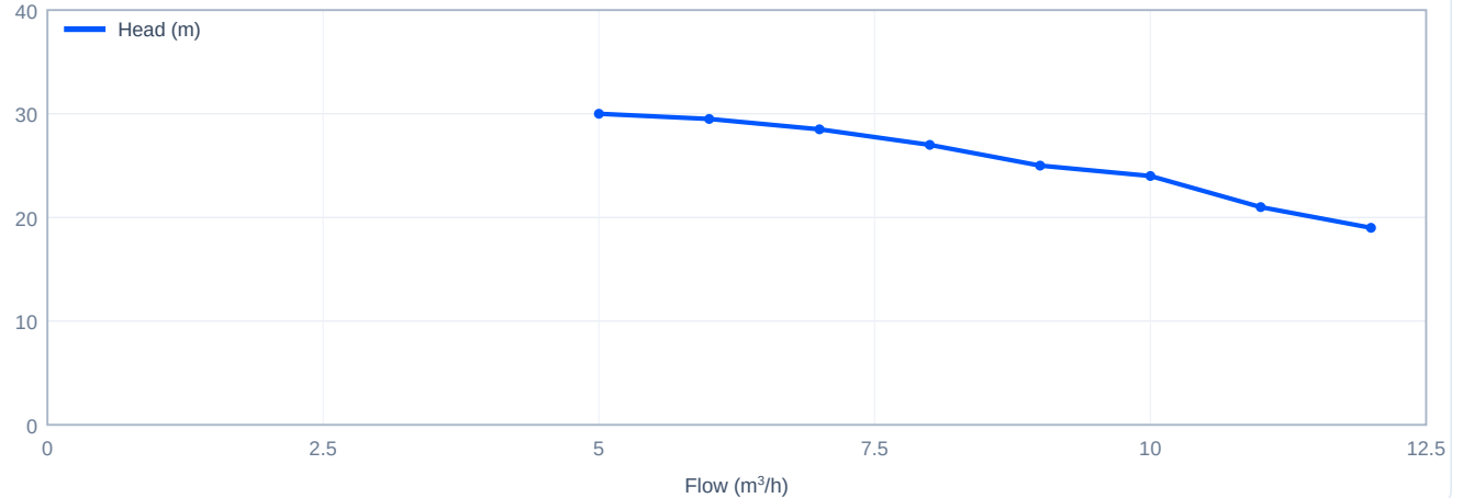
Head versus flow - CDLK8-30/3, 50 Hz
