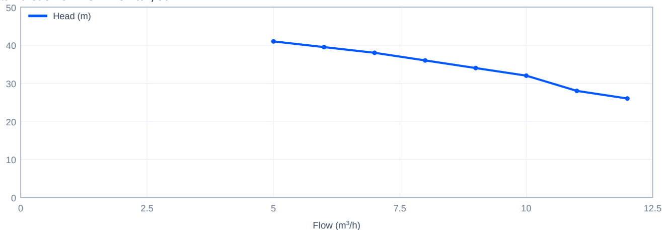
Head versus flow - CDLK8-40/4, 50 Hz
