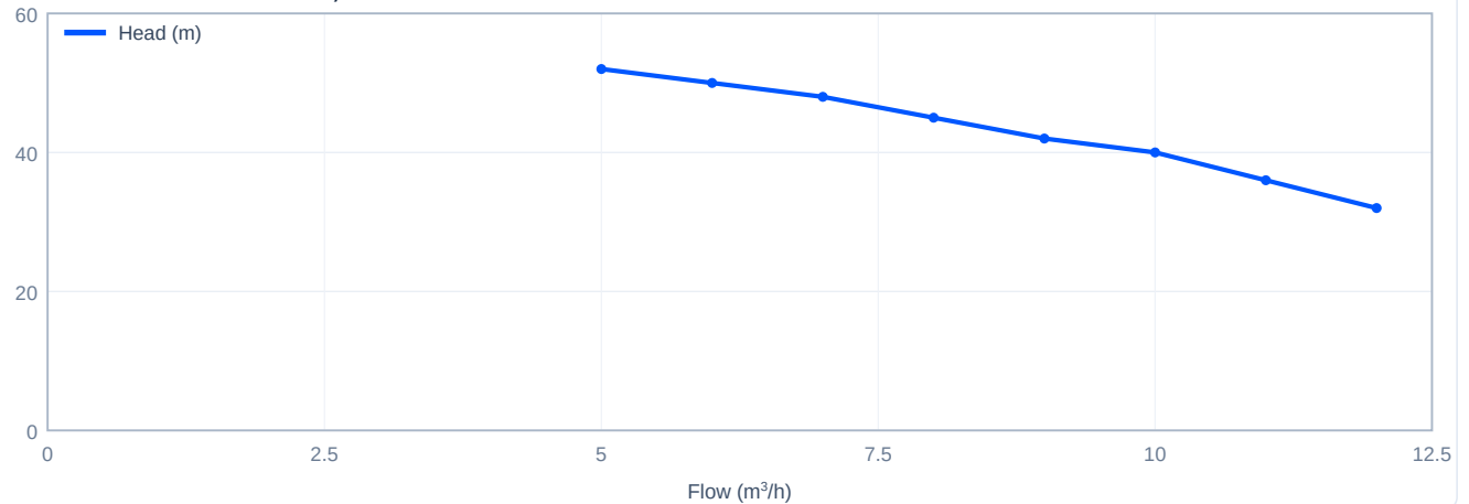
Head versus flow - CDLK8-50/5, 50 Hz
