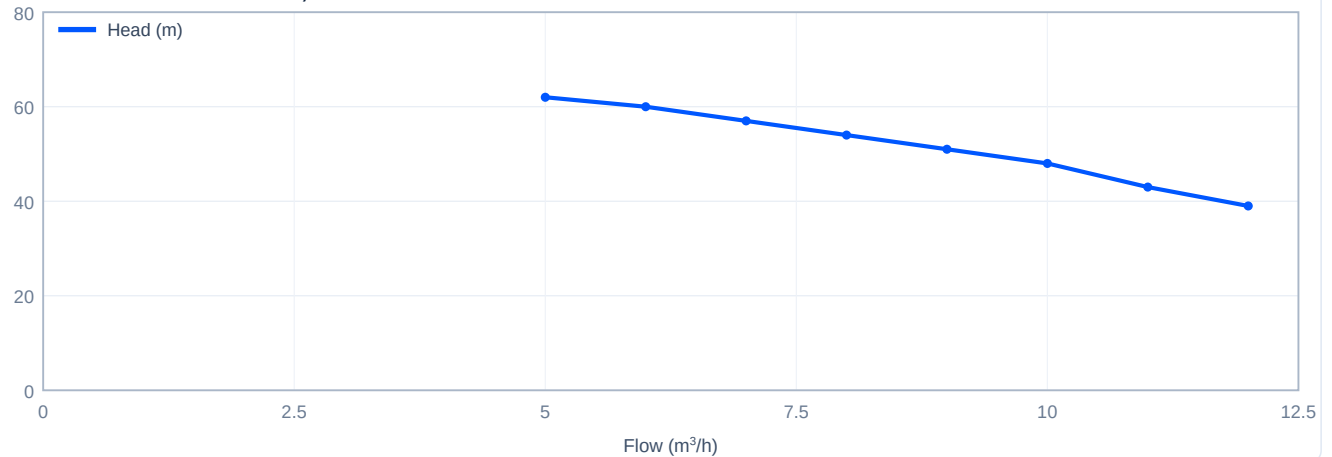
Head versus flow - CDLK8-60/6, 50 Hz
