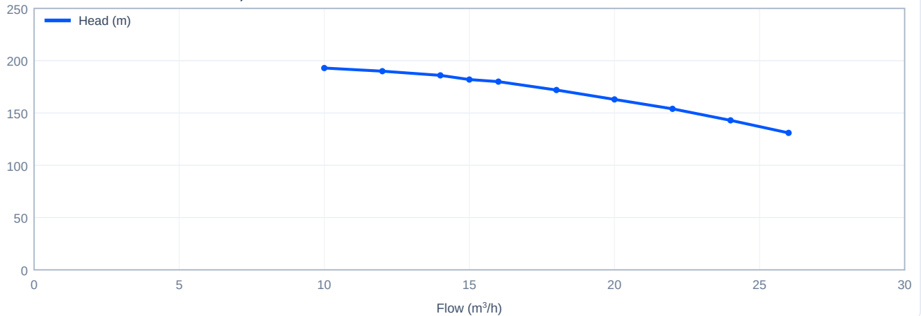
Head versus flow - CDLK15-100/10, 60 Hz
