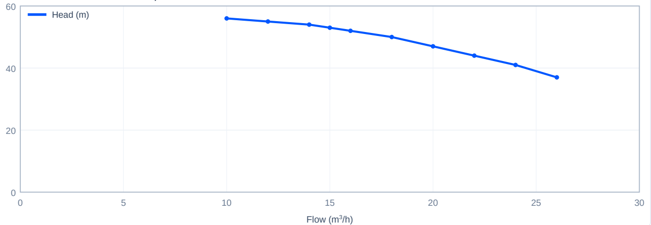
Head versus flow - CDLK15-30/3, 60 Hz
