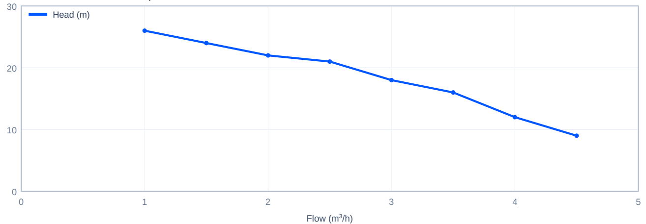
Head versus flow - CDLK2-20/2, 60 Hz
