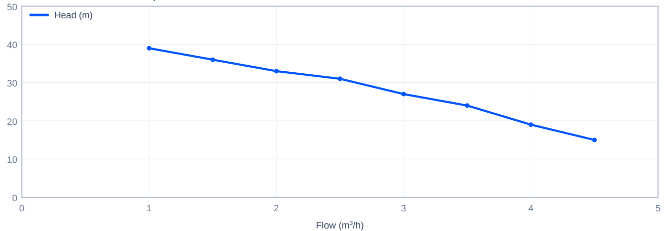
Head versus flow - CDLK2-30/3, 60 Hz
