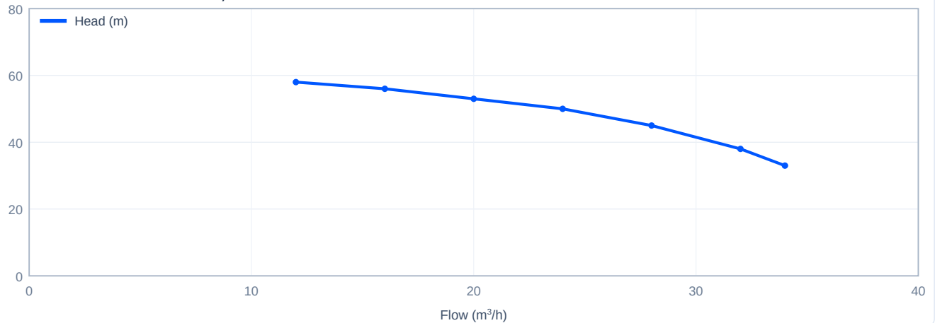
Head versus flow - CDLK20-30/3, 60 Hz
