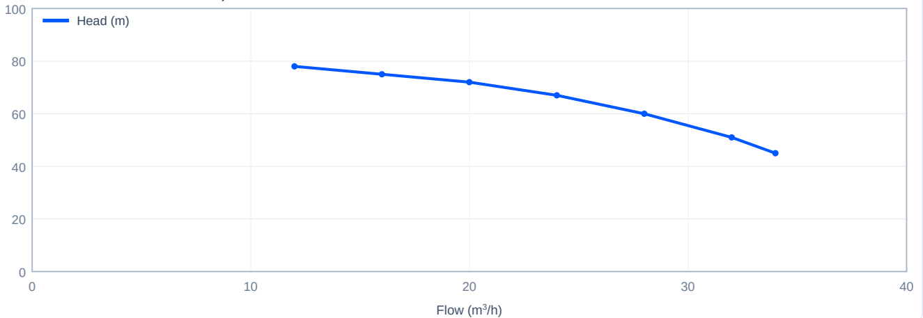
Head versus flow - CDLK20-40/4, 60 Hz
