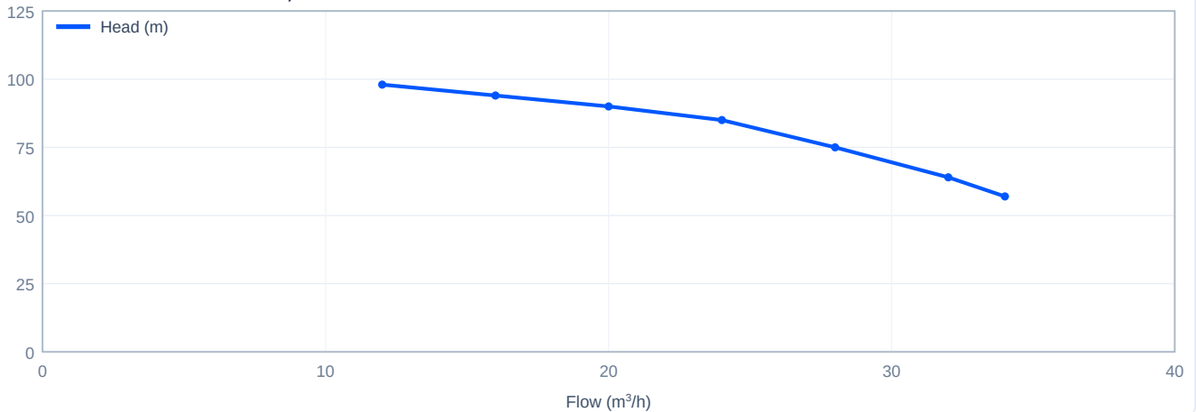
Head versus flow - CDLK20-50/5, 60 Hz
