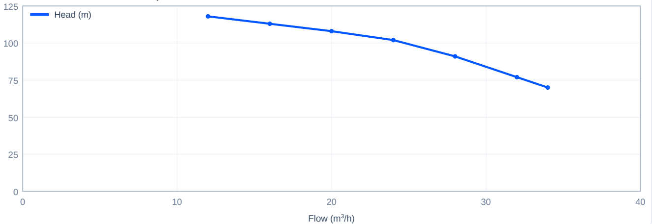
Head versus flow - CDLK20-60/6, 60 Hz
