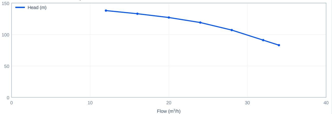
Head versus flow - CDLK20-70/7, 60 Hz
