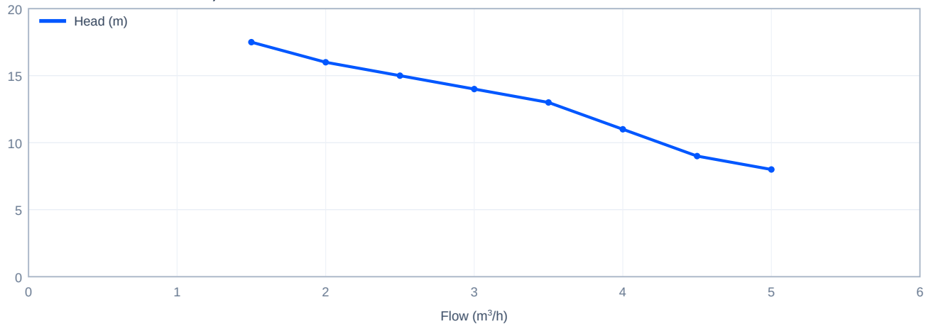
Head versus flow - CDLK3-20/2, 60 Hz
