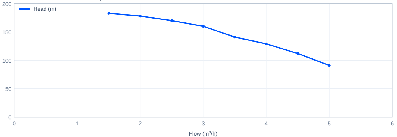
Head versus flow - CDLK3-210/21, 60 Hz
