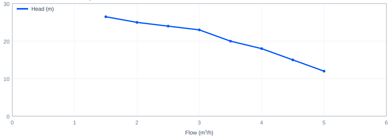
Head versus flow - CDLK3-30/3, 60 Hz
