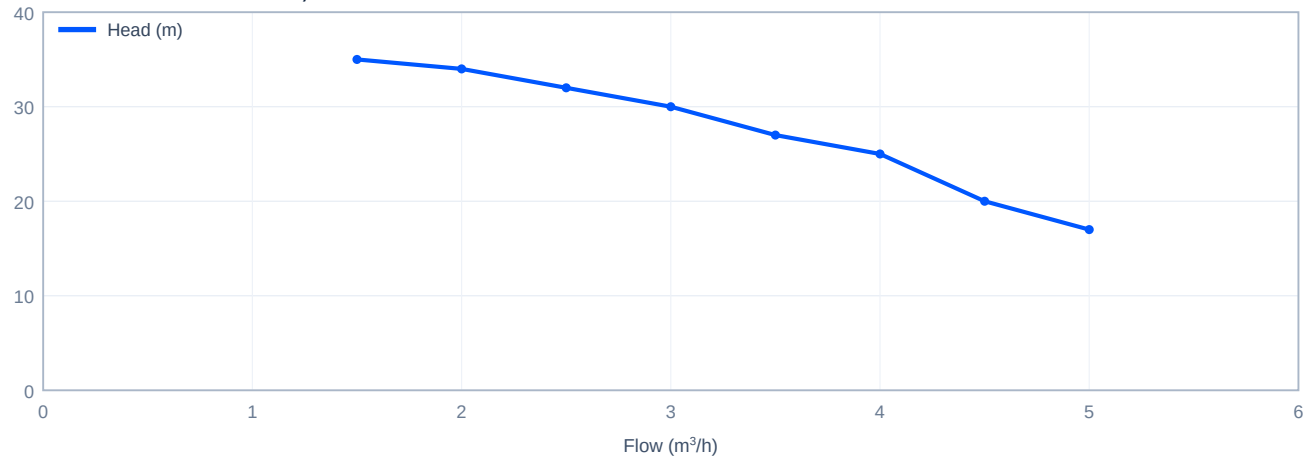
Head versus flow - CDLK3-40/4, 60 Hz
