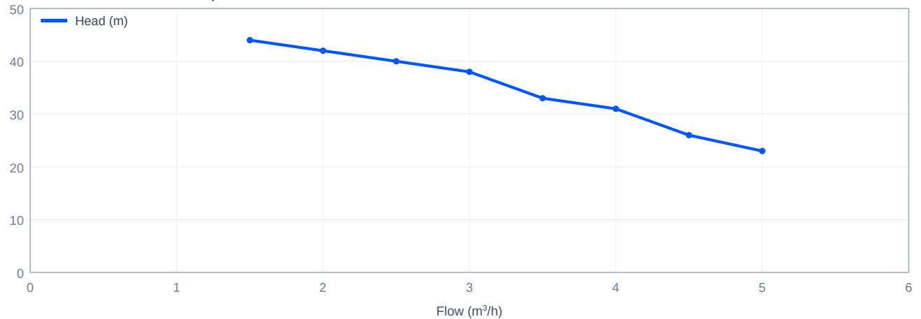
Head versus flow - CDLK3-50/5, 60 Hz
