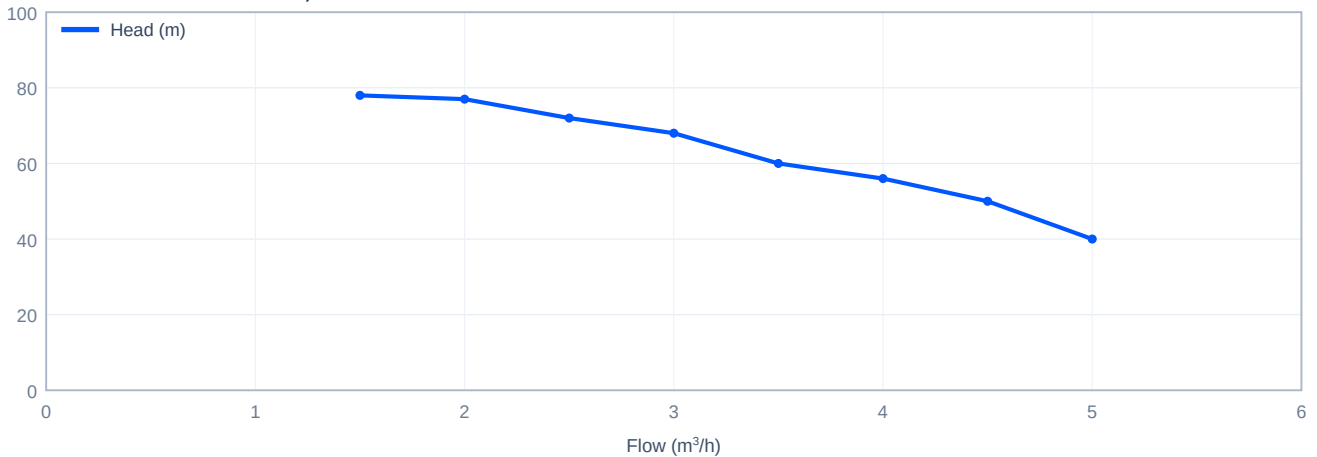
Head versus flow - CDLK3-90/9, 60 Hz
