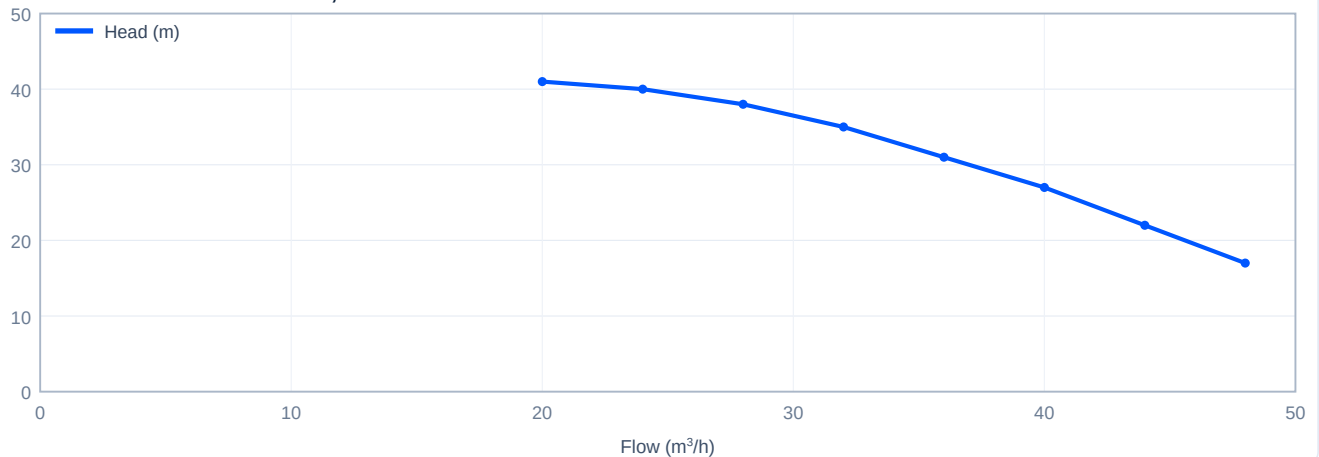
Head versus flow - CDLK32-20/2-2, 60 Hz
