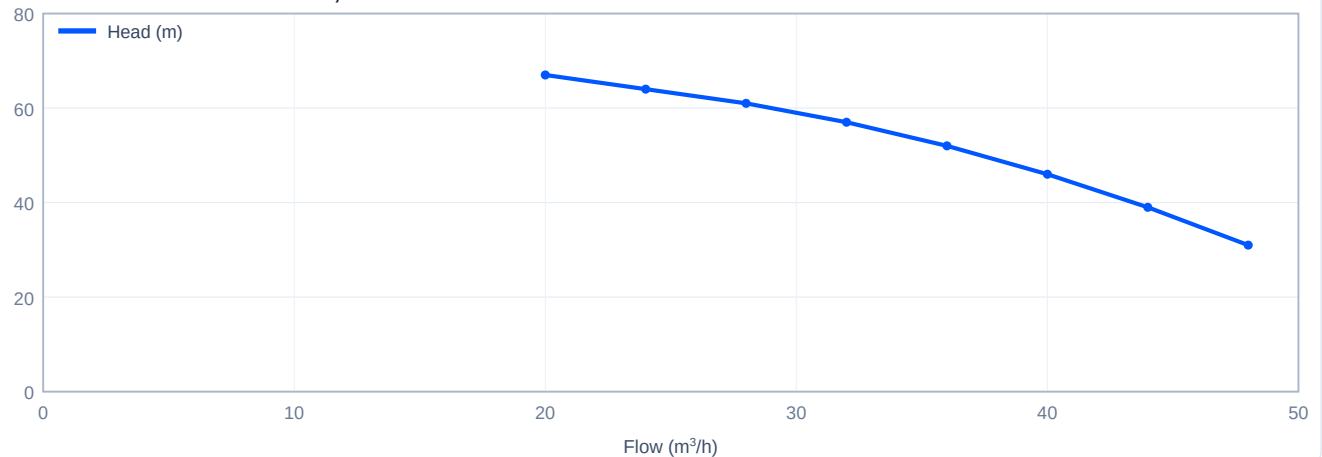
Head versus flow - CDLK32-30/3-2, 60 Hz
