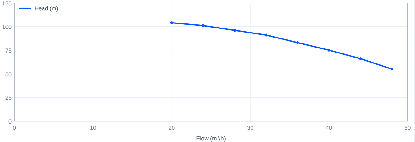
Head versus flow - CDLK32-40/4, 60 Hz
