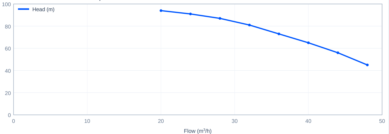
Head versus flow - CDLK32-40/4-2, 60 Hz
