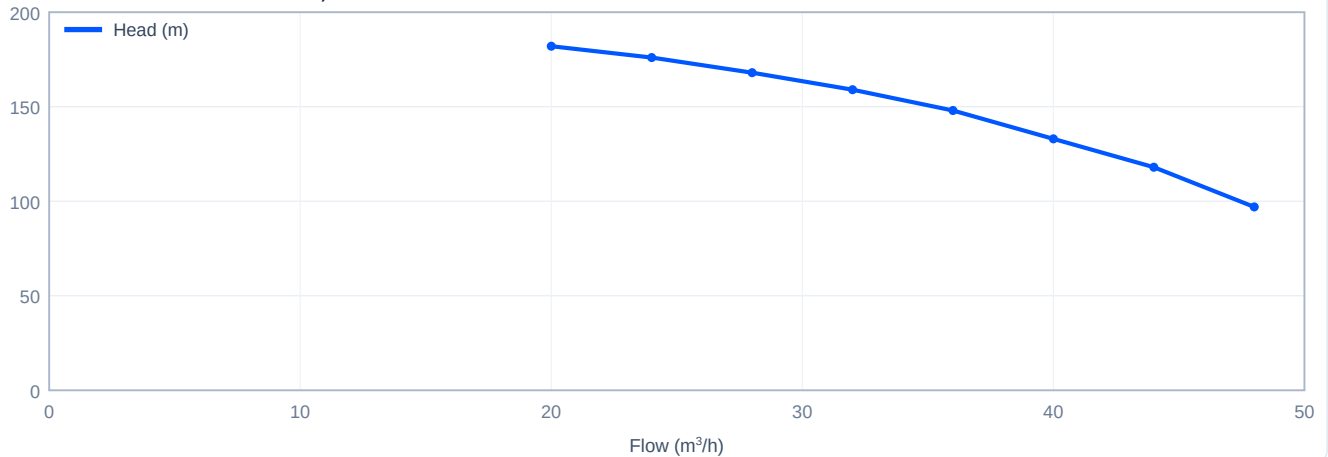
Head versus flow - CDLK32-70/7, 60 Hz
