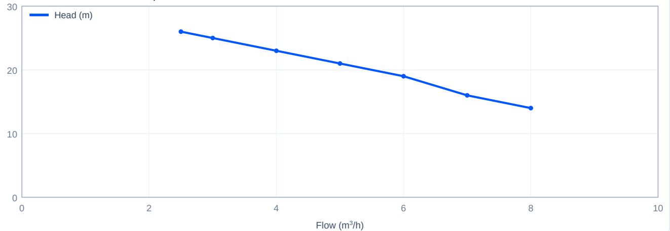
Head versus flow - CDLK4-20/2, 60 Hz
