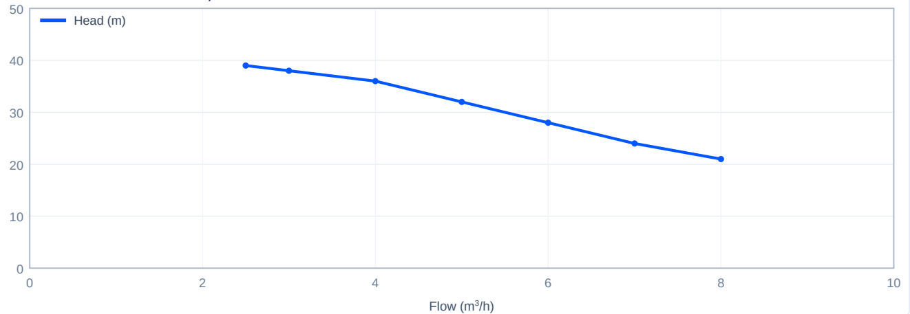
Head versus flow - CDLK4-30/3, 60 Hz
