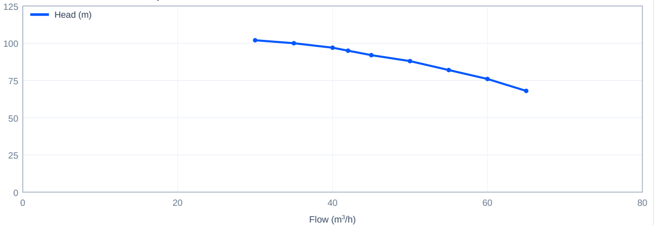
Head versus flow - CDLK42-30/3, 60 Hz
