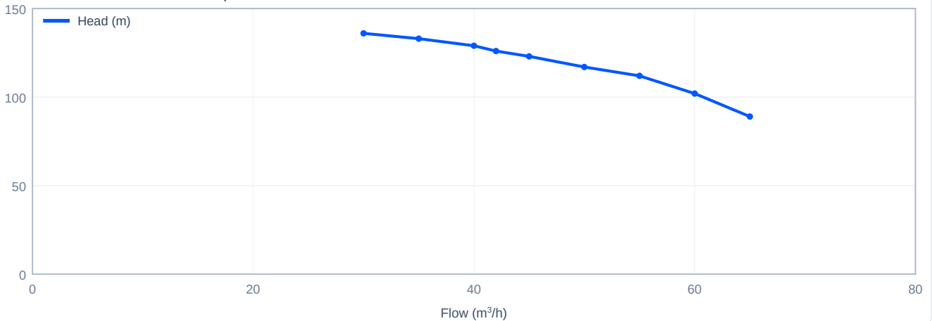
Head versus flow - CDLK42-40/4, 60 Hz
