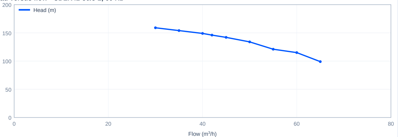
Head versus flow - CDLK42-50/5-2, 60 Hz
