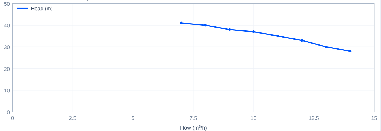
Head versus flow - CDLK8-30/3, 60 Hz
