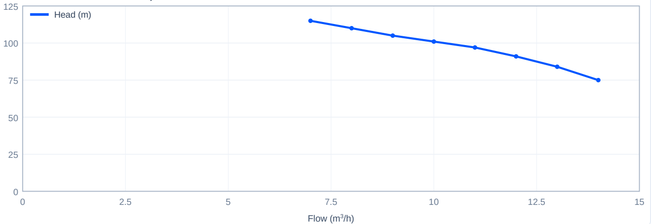
Head versus flow - CDLK8-80/8, 60 Hz
