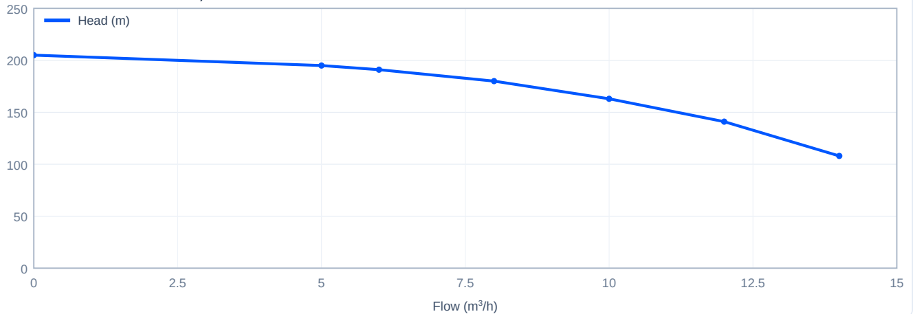
Head versus flow - CDM10-18, 50 Hz
