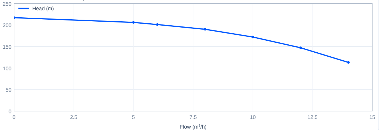
Head versus flow - CDM10-19, 50 Hz
