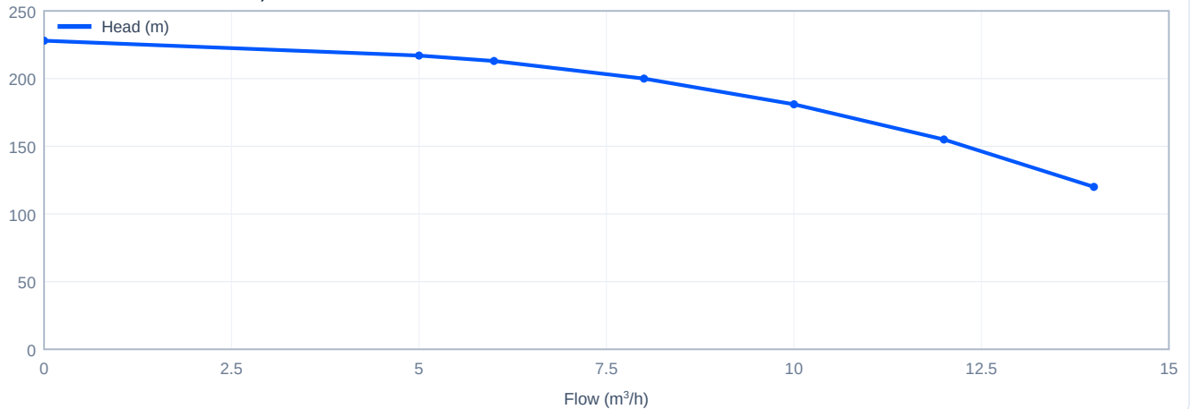
Head versus flow - CDM10-20, 50 Hz
