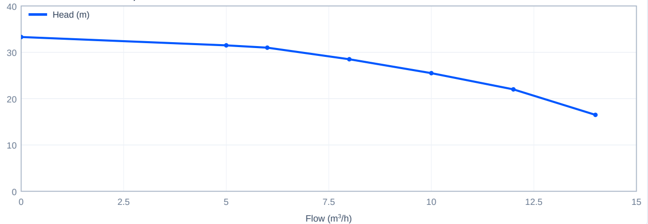
Head versus flow - CDM10-3, 50 Hz
