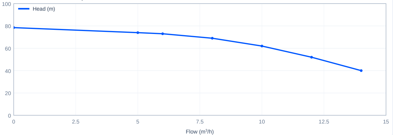
Head versus flow - CDM10-7, 50 Hz
