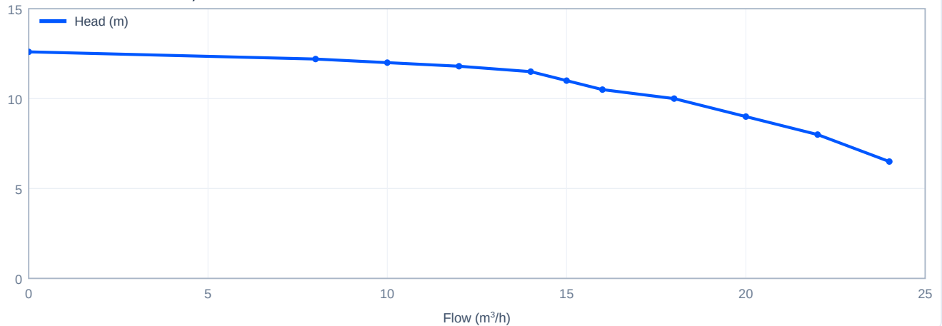
Head versus flow - CDM15-1, 50 Hz
