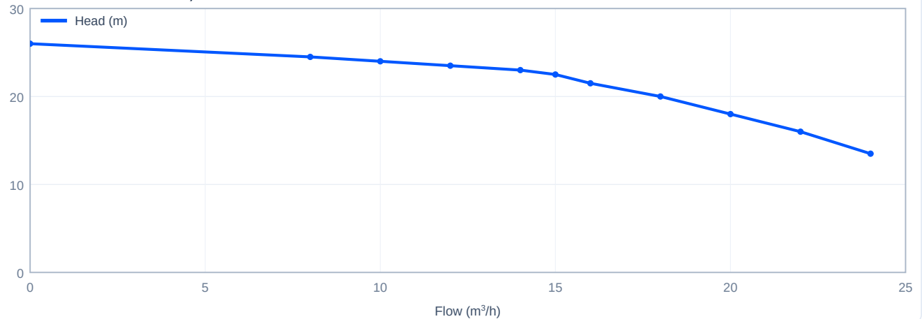
Head versus flow - CDM15-2, 50 Hz
