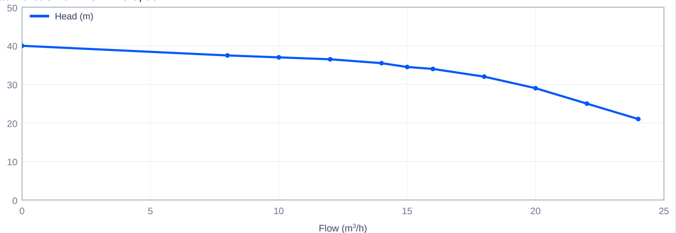
Head versus flow - CDM15-3, 50 Hz
