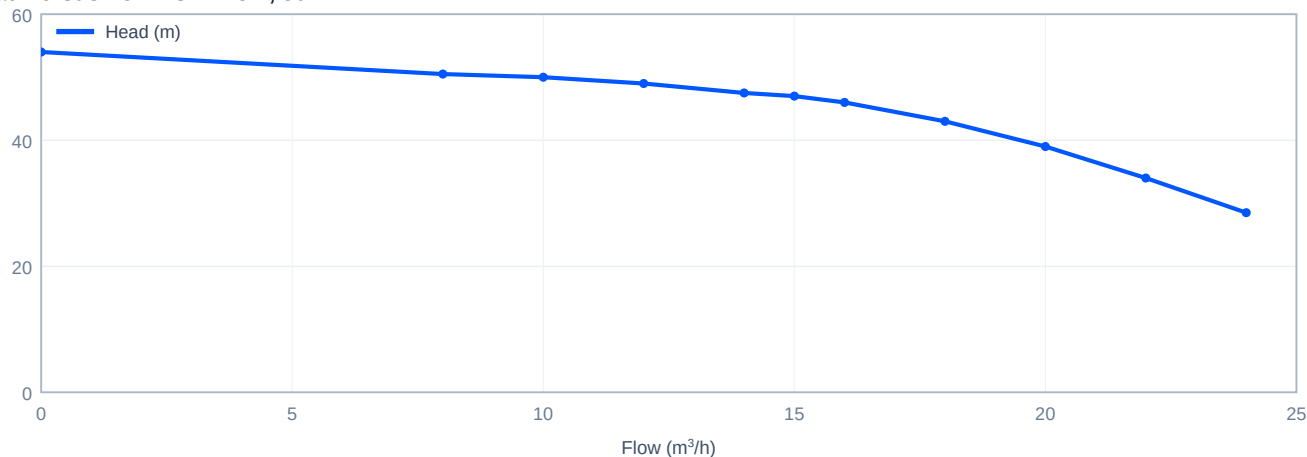
Head versus flow - CDM15-4, 50 Hz
