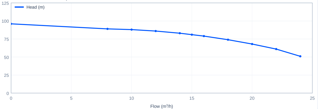
Head versus flow - CDM15-7, 50 Hz
