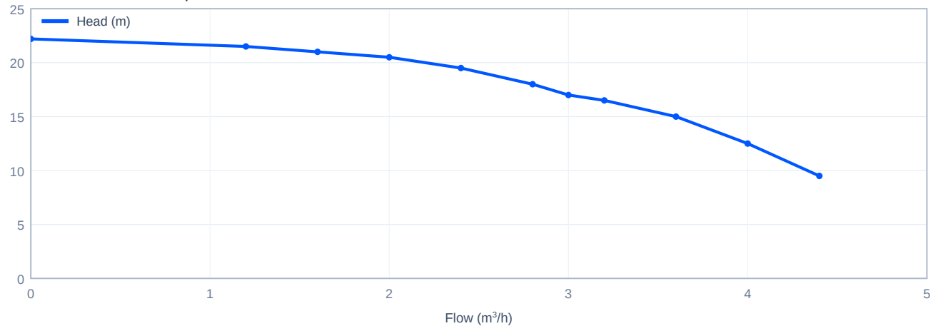
Head versus flow - CDM3-3, 50 Hz
