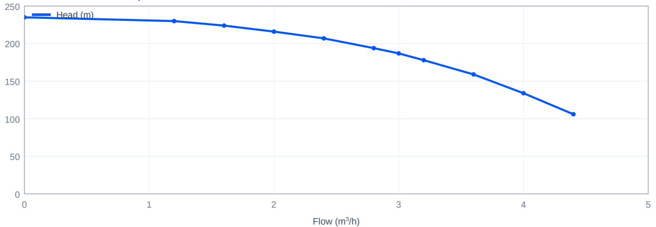
Head versus flow - CDM3-31, 50 Hz
