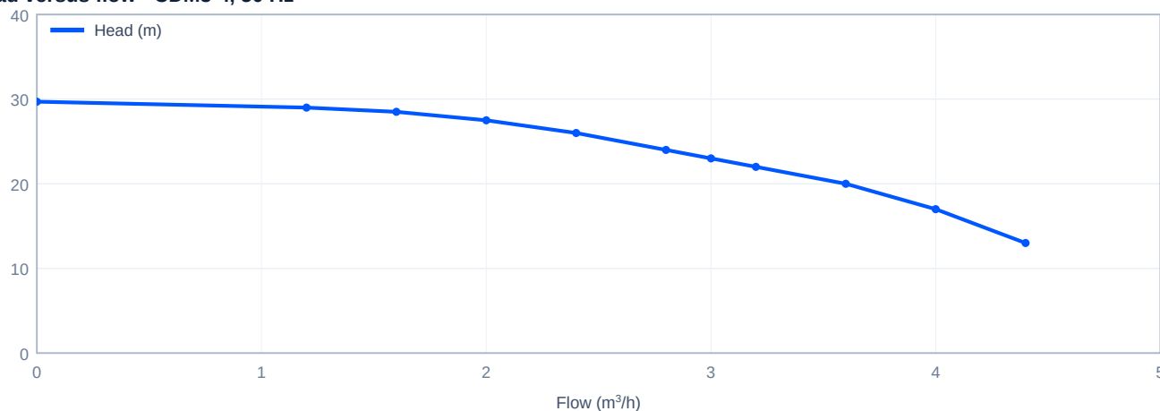
Head versus flow - CDM3-4, 50 Hz
