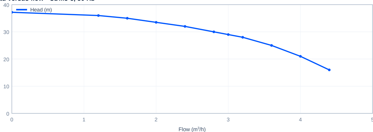
Head versus flow - CDM3-5, 50 Hz
