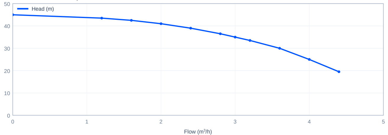
Head versus flow - CDM3-6, 50 Hz
