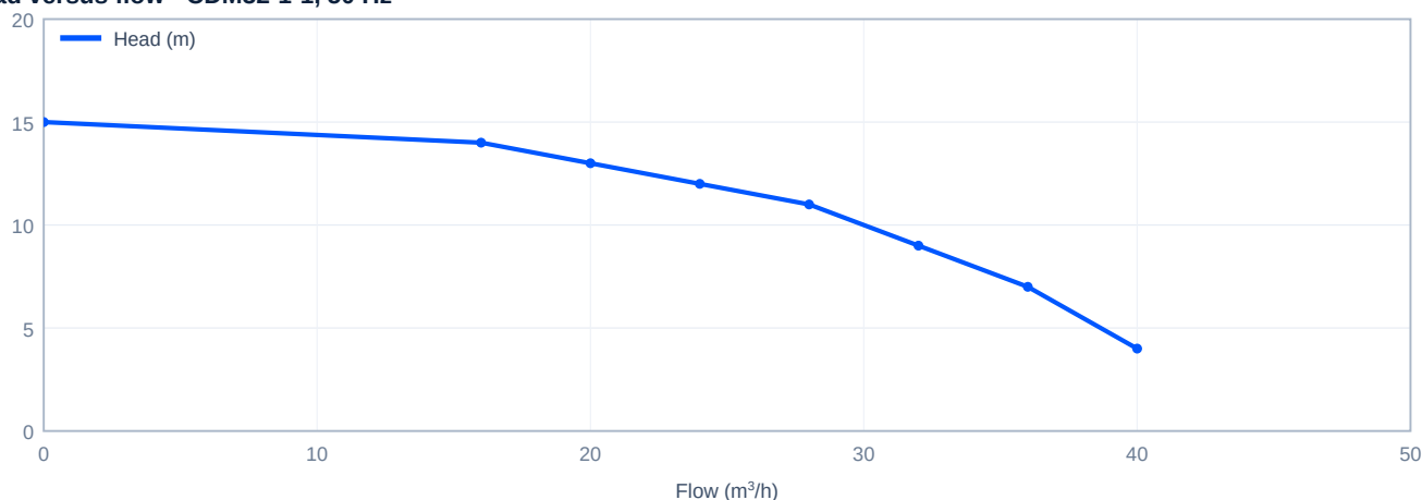
Head versus flow - CDM32-1-1, 50 Hz
