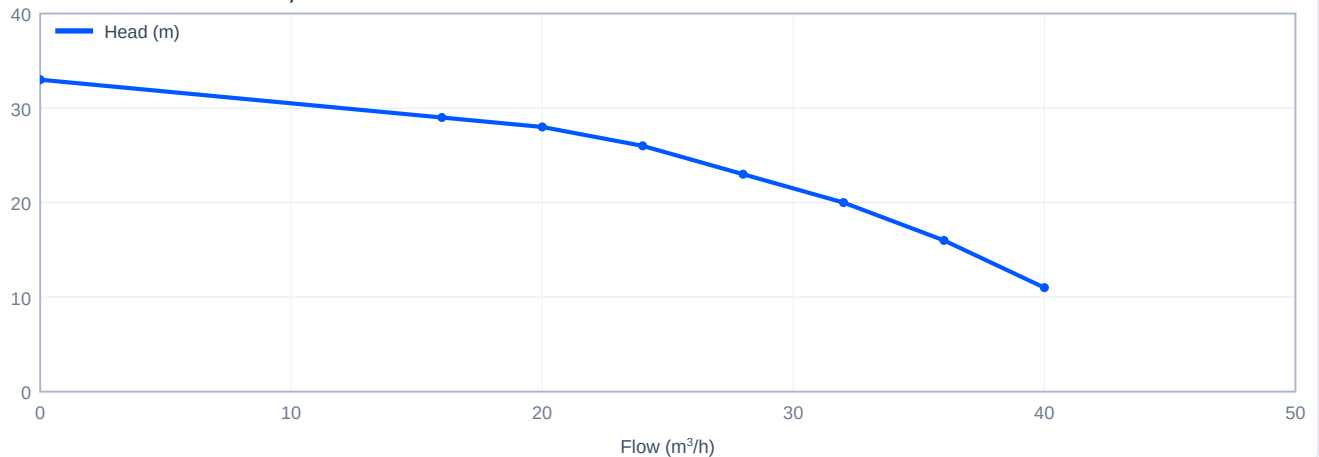
Head versus flow - CDM32-2-2, 50 Hz
