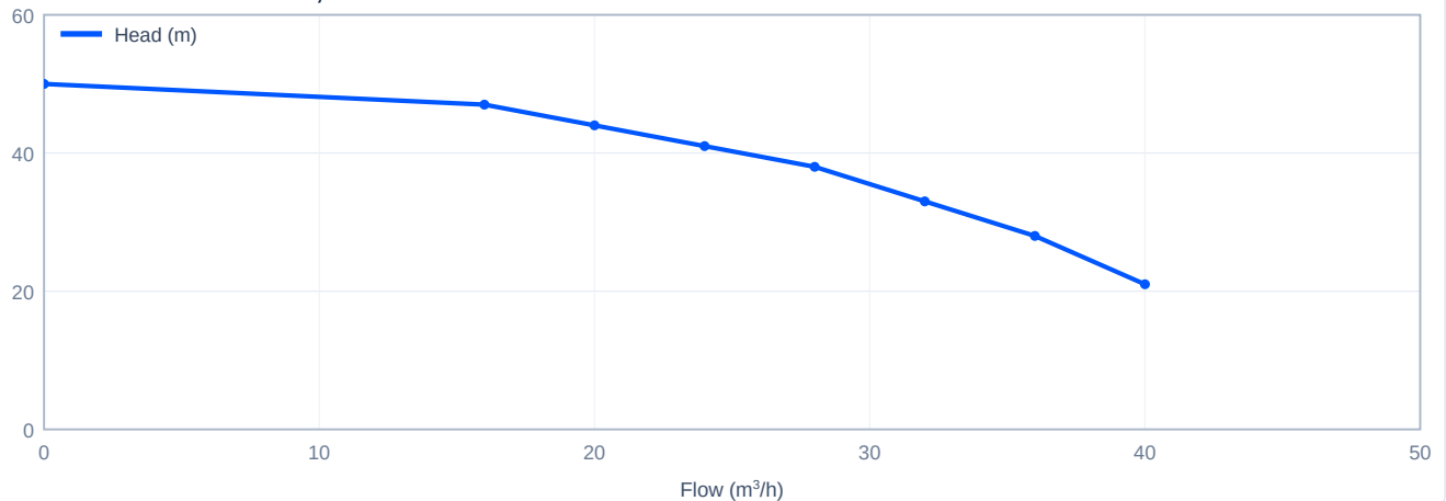
Head versus flow - CDM32-3-2, 50 Hz
