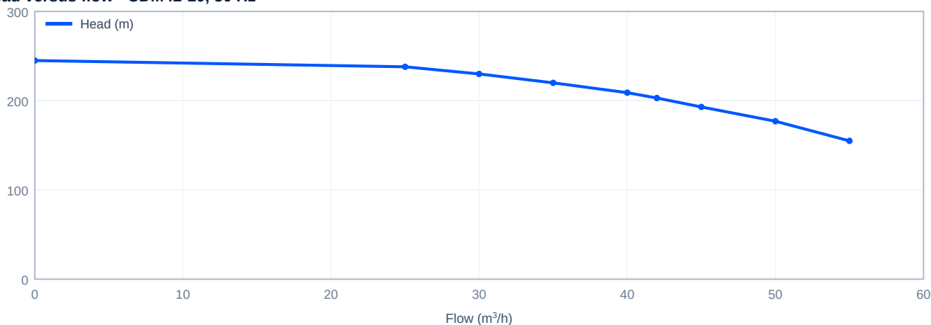
Head versus flow - CDM42-10, 50 Hz
